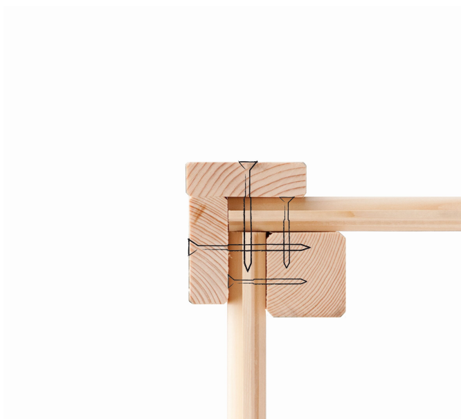
19mm PROFILE
