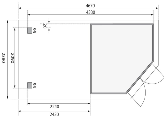
Fundamentplan (in mm)
